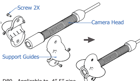
Figure 12. Install 80 Support Guides
