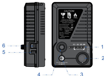
Figure 4. Battery pack
