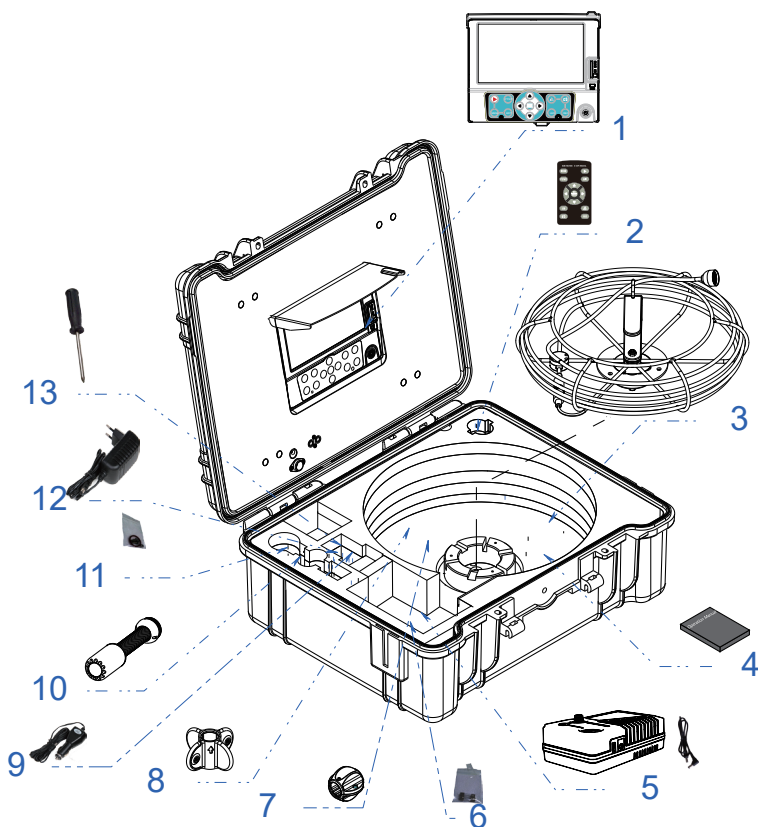
Figure 6. Package Contents
