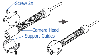
D46 Applicable to 2.5"-3.5" pipe.
